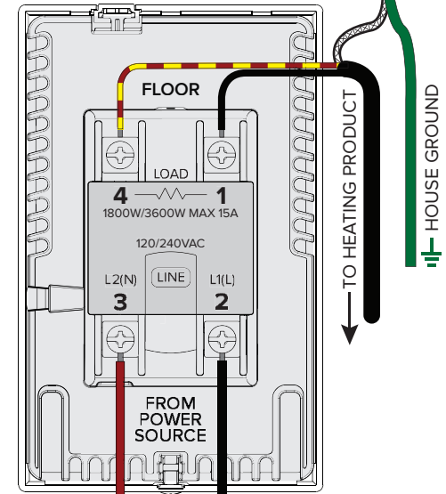
REAR OF THE USG BASE
