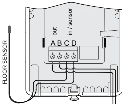
FRONT OF THE THERMOSTAT BASE
