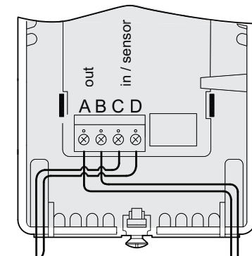
FRONT OF THE BASE
