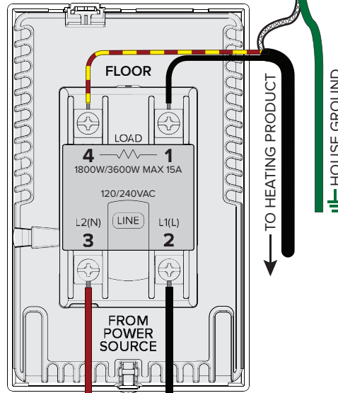
REAR OF THE USG BASE
