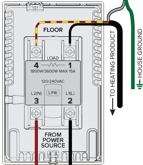
REAR OF THE THERMOSTAT BASE
